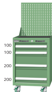
EA-7041MA H1380xW566xD640 72pcs/20ft ; 152pcs/40ft EB-7041MA H1380xW718xD640 54pcs/20ft ; 114pcs/40ft
